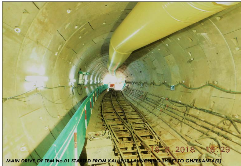
Fig. 8 Tunneling Work from Kalupur launching shaft to Gheekanta
